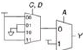
Figure 2.87 Multiplexer circuit
